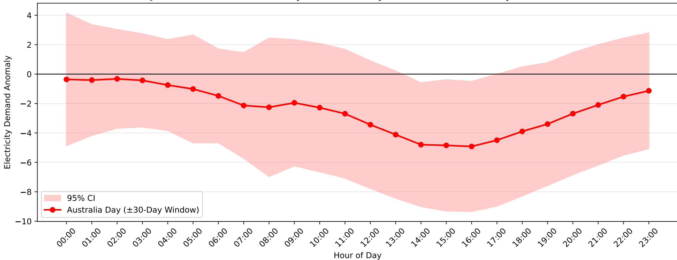
Jesmond Demand Anomaly: Australia Day (2004–2017, \pm 30 -Day Window)
